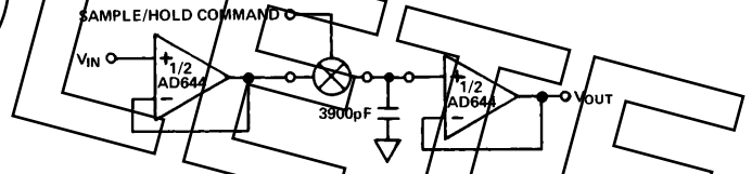
Figure 29. Sample and Hold Circuit
